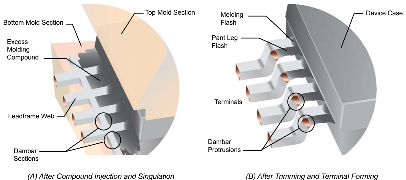
Figure 2. Molding Flash. Case molds have upper and lower halves, which allow flash, the small amount of excess molding compound that remains after the device is ejected from the mold and the device is singulated and trimmed. Interlead flash is allowed between the case and the dambar protrusion, and is away from the critical soldering areas.
