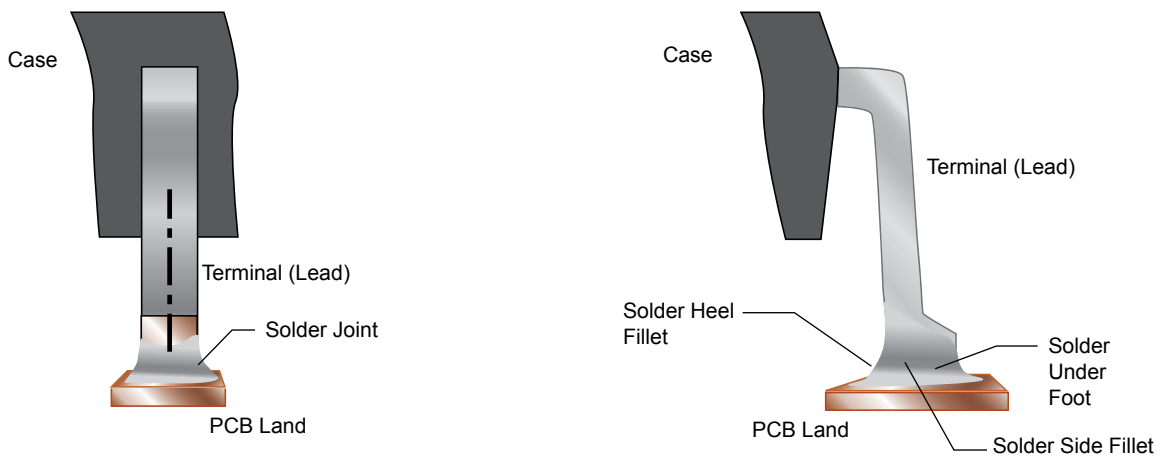
Figure 7. Mini Gull Wing (L Lead) Solder Joint. Although this type of terminal has the basic shape of a full gull-wing terminal (IPC-A-610 §8.2.5.), the truncated foot requires additional attention for joint strength, such as the specification for the butt terminal joint (IPC-A-610 §8.2.8). Although high-reliability (class 3) is not defined for the butt joint, similar minimal rules, including no toe overhang, a minimum 75% terminal width fillet, as well as practical rules of no terminal lateral overhang, and maximum heel fillet, should be observed.
