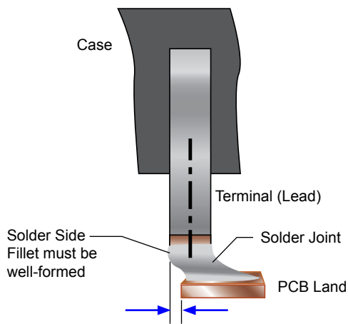
Figure 4. Gull Wing Solder Joint. Although a maximum overhang of 25% of the terminal width or 0.5 mm, whichever is less, is allowed for a high-reliability (IPC class 3) assembly (IPC-A-610 §8.2.5), a fillet on the the outboard side of the terminal is always required.
