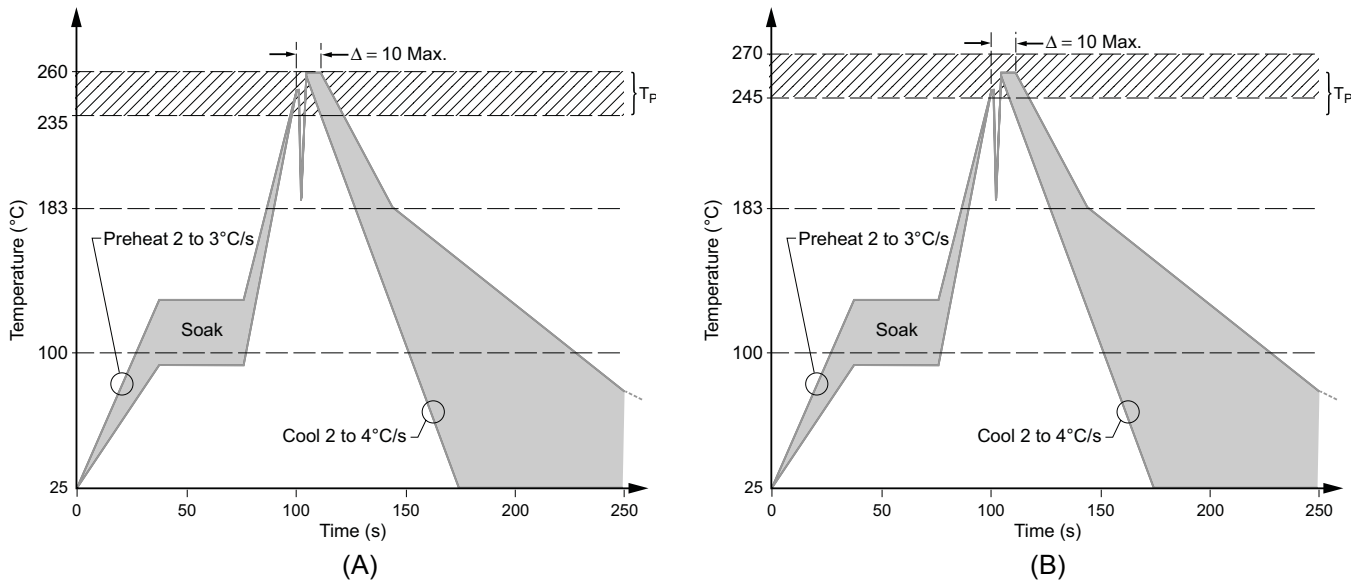
Figure 10. Solder Reflow Profile for Through-Hole Wave Solder Using (A) Traditional Tin-Lead Solder and (B) Pb-free solder.
