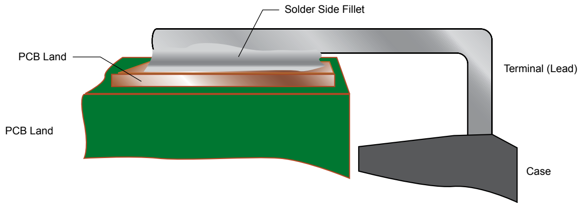
Figure 6. Bent Lead Solder Joint. For straight terminals parallel to the PCB, such as an SIP with leads bent around the edge of a PCB, no lateral overhang of the terminal should be permitted for a high-reliability (IPC class 3) assembly. Solder underneath the lead should be thick, and a wetted fillet should be evident between the lead and the lands (IPC-A-610 §8.2.5.7).
