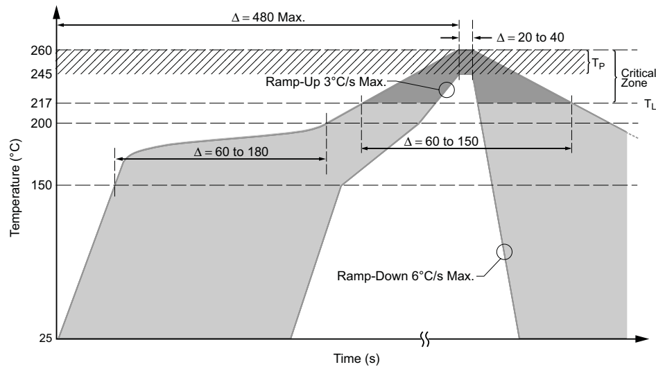
Figure 9. Solder Reflow Profile for SMD Using Lead (Pb) Free Solder. The typical acceptable maximum temperature range, T_P , is 245°C to 260°C. Temperatures refer to upper surface of the package case.
