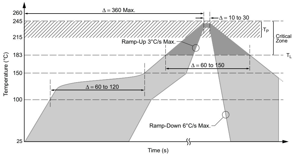
Figure 8. Solder Reflow Profile for SMD Using Traditional Tin-Lead Solder. The typical acceptable maximum temperature range, T_P , is 215°C to 245°C. Temperatures refer to upper surface of the package case.
